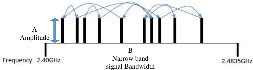
Figure.2 With Frequency Hopping Spread Spectrum, the signal is transmitted on different frequencies at intervals to spread the signal across a relatively wide operating band.
