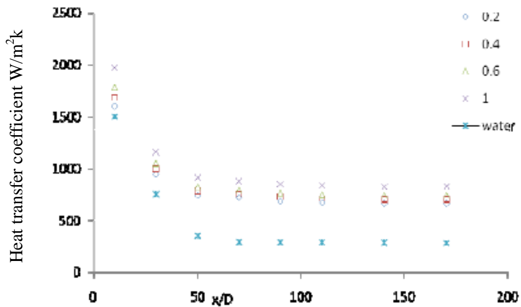
Figure 8: Coefficient of thermal transmission of metallic Cu nanofluids along the pipe at Re 1300.
