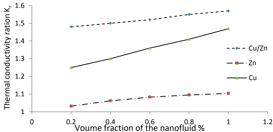
Figure 5. Volume fraction against thermal conductivity ratio of different type nanofluids.
