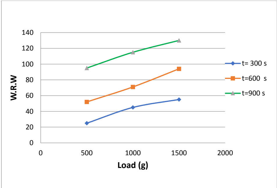
Figure 1. Relationship between Wear Rate by Volume (W.R.W) and load for Aluminum Sample at Different Test Time
