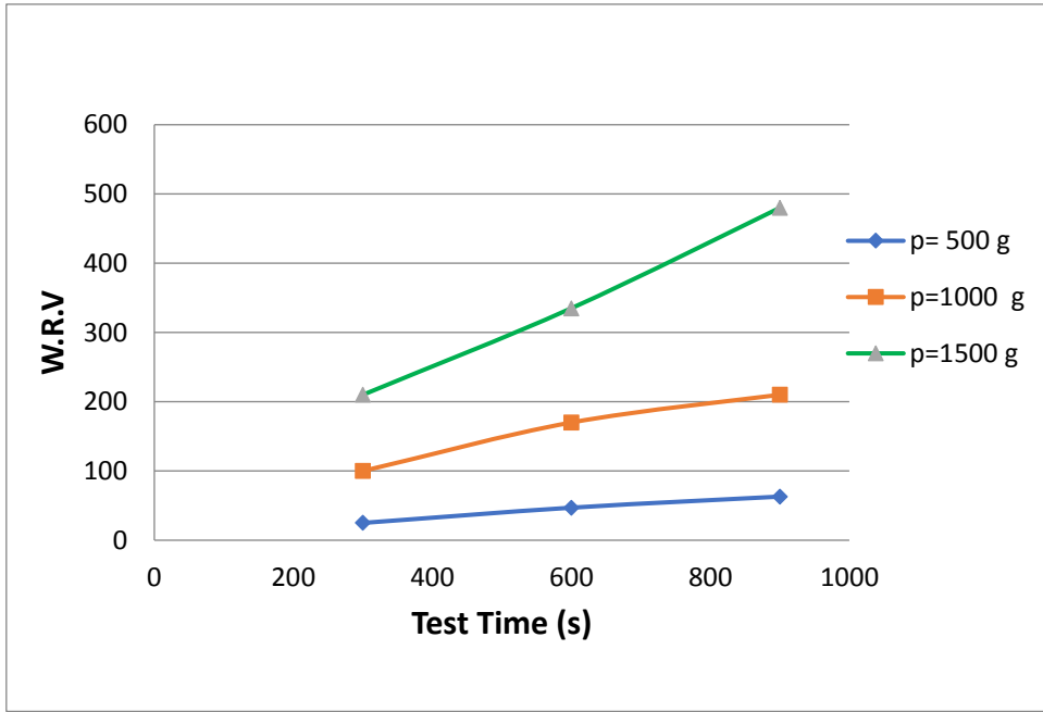
Figure 4. Relationship between Wear Rate by Volume (W.R.V) and Test Time for Aluminum Sample at Different Test Time
