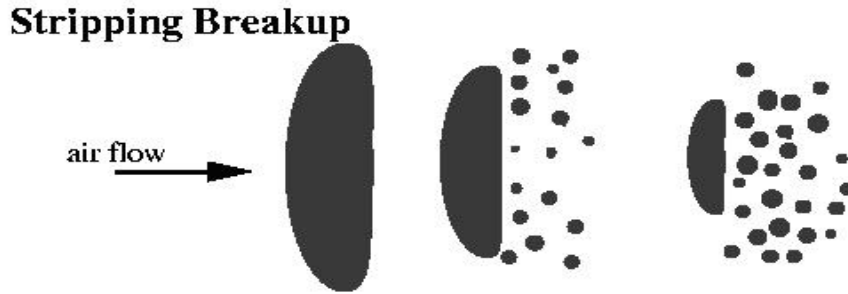
Figure 2: Stripping breakup ( We_g > \sqrt{Re} )
