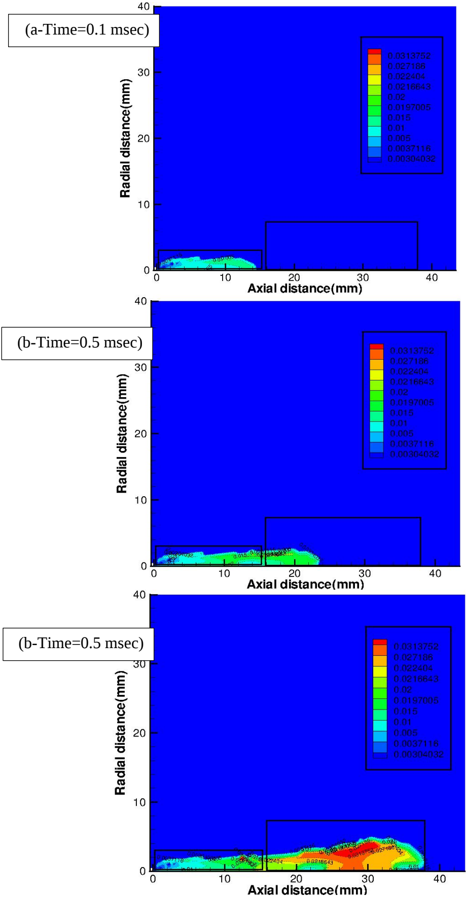
Figure 10: Contour plots of the stable breakup droplet diameter at different time.
