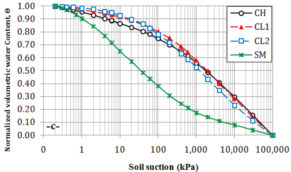
Fig. 6: Soil water characteristic curve of the different soils in terms: a- Gravimetric, b- Volumetric and c- Normalized volumetric water content, versus soil suction
