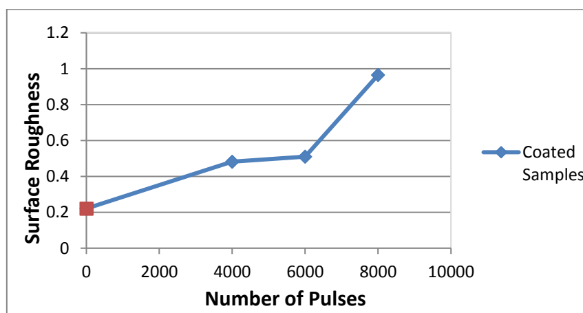
Figure (11): The Effect of Laser Pulses on Surface Roughness of HA coating.
