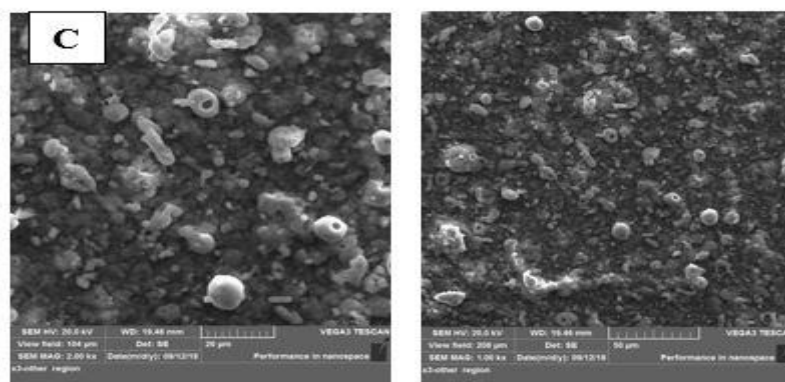
Figure (6): SEM Micrographs of Samples (A) B1, (B) B2, and (C) B3
