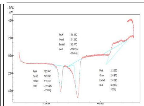
Fig 11. Show the DSC curve of (30LDPE:70 aPP)
