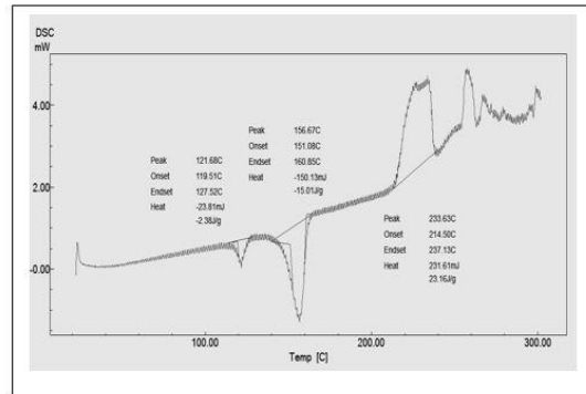
Fig (9) show the DSC curve of pure PP
