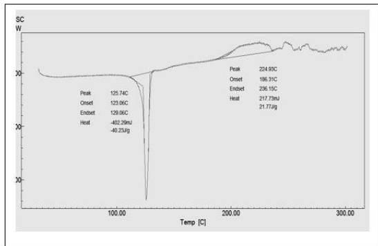
Fig (8) show the DSC curve of pure LDPE
