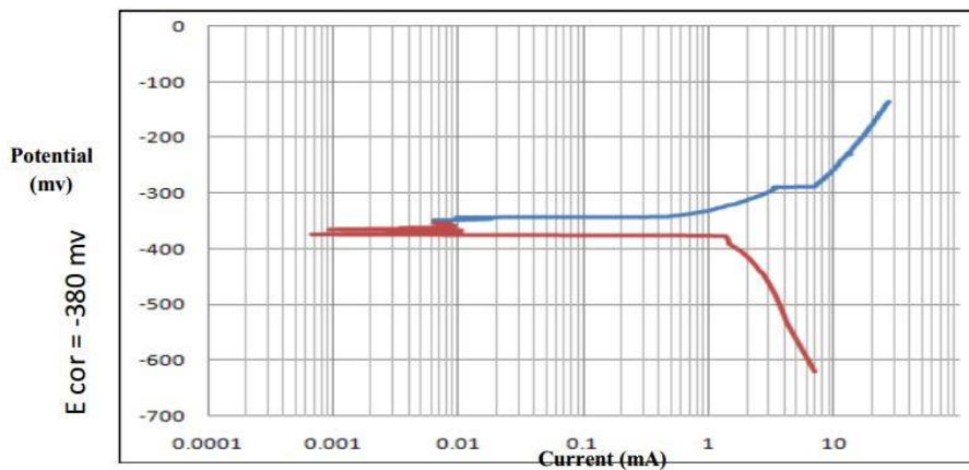
Figure (14): Potentiostatic Polarization curve of alloy (B). I_{cor} = 0.9411 \mu A
