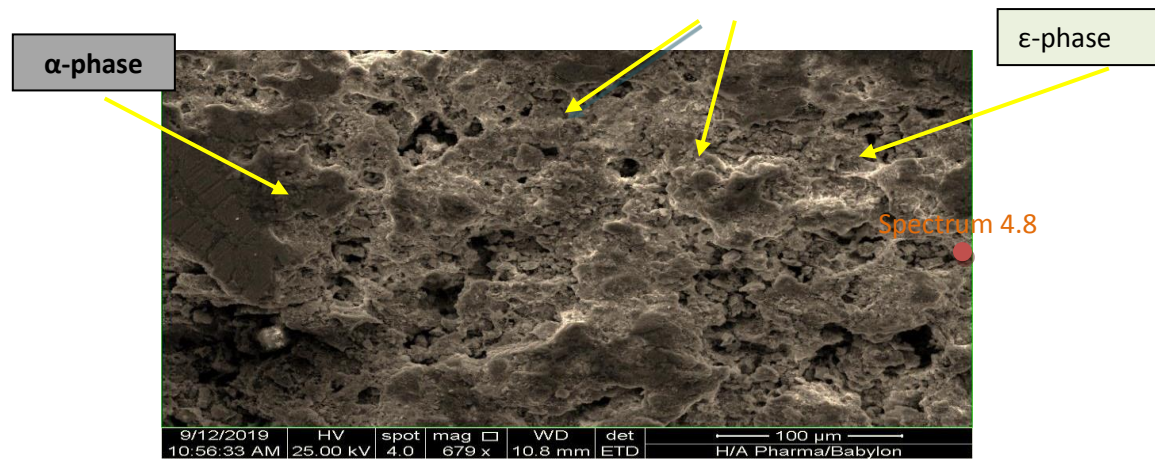
Figure (7): SEM-Image Represent Morphology of Base Alloy (A).
