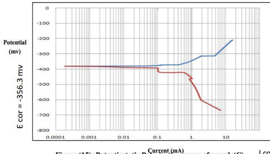
Figure (15): Potentiostatic Polarization curve of sample(C).
